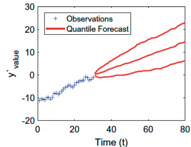
Regression
